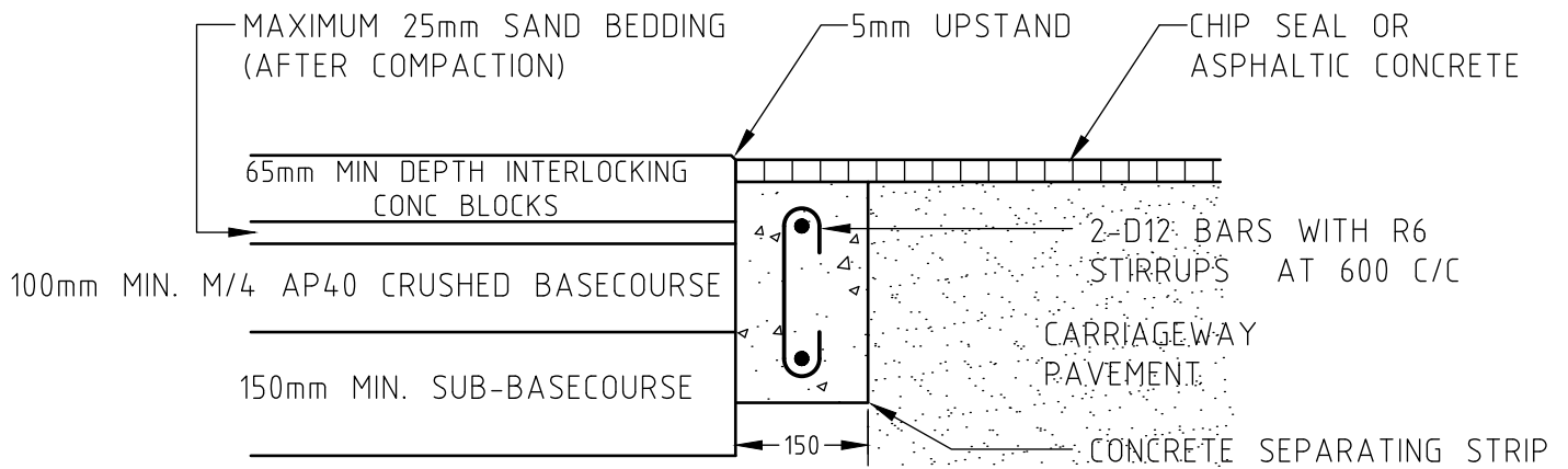
CARRIAGEWAY THRESHOLDS (LONGITUDINAL SECTION)
