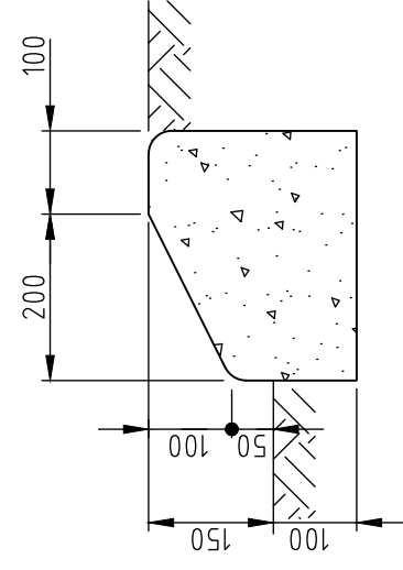
MOUNTABLE KERB
