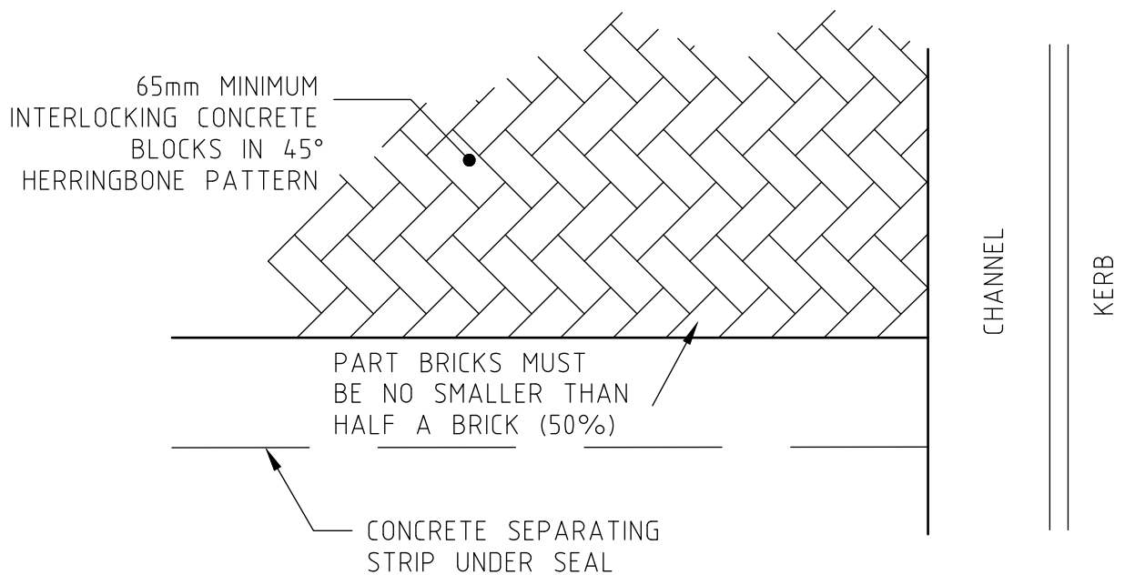
CARRIAGEWAY THRESHOLDS PART PLAN
