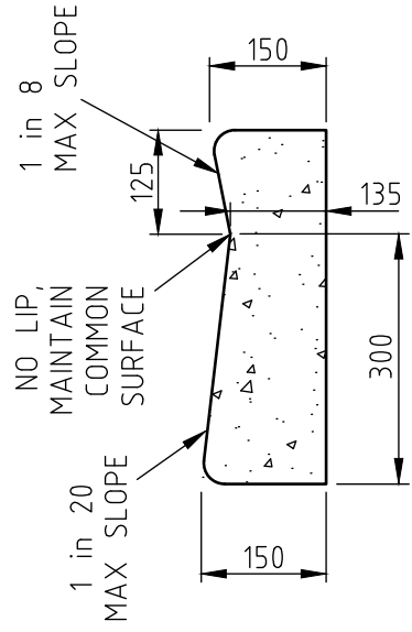
PRAM CROSSING
