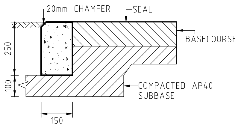
INSET 'A'
