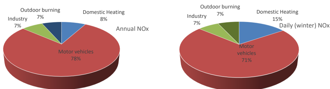
Figure 7.3: Relative contribution of sources to daily winter and annual average CO, emissions in Brightwater
