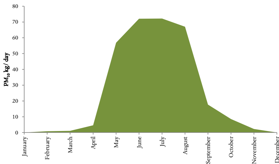
Figure 3.4: Monthly variations in PM 10 emissions from domestic heating in Brightwater.
