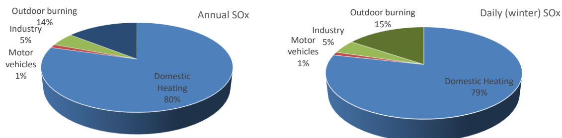
Figure 7.4: Relative contribution of sources to annual (left) and daily winter (right) NOx emissions in Brightwater.
